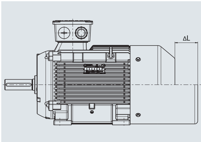
Motor with separately driven fan
