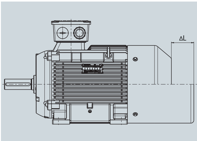
Motor with separately driven fan
