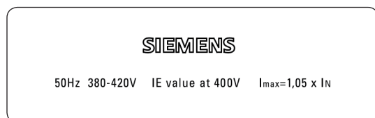
Example of Voltage Sticker (Option code B07)
